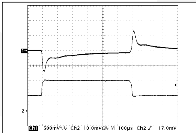
Figure 11: Output voltage response to step-change in load current (50%-100%-50% of Iout(max)). Load cap: 1μF ceramic cap and 10μF, 100 mΩ ESR tantalum cap. Ch 1: Vout (500mV/div). Ch 2: Iout (2A/div).
