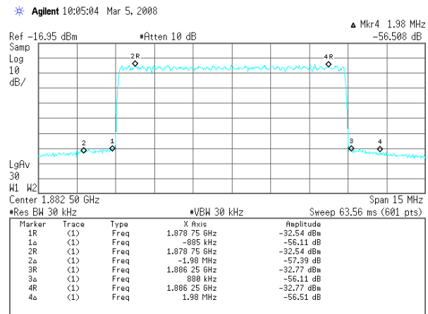
Spurious Emission @ Fc 1882.5MHz, CDMA 7FA, 32dBm
