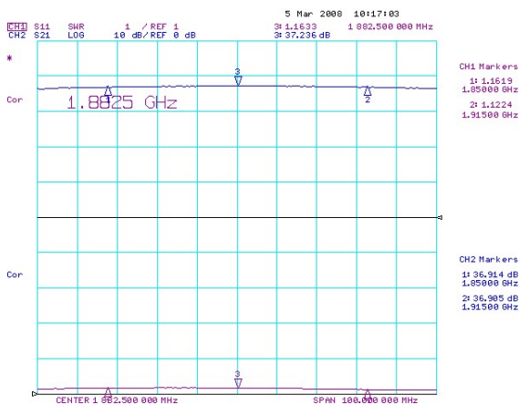
Gain & S11
