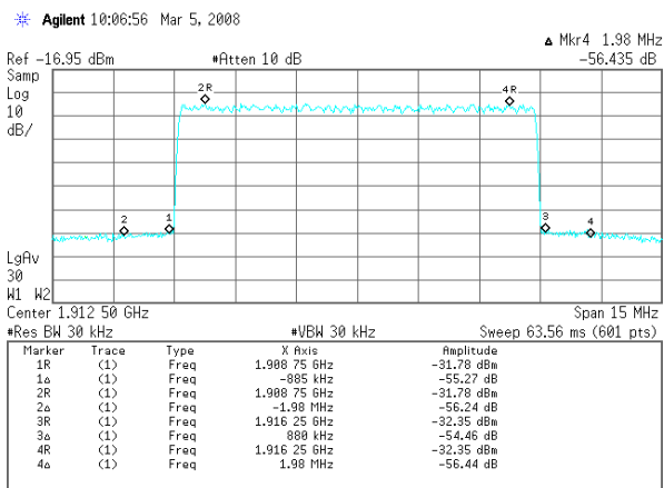
Spurious Emission @ Fc 1912.5MHz, CDMA 7FA, 32dBm
