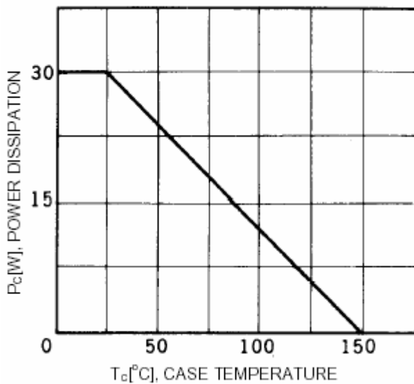
Fig.7 Power Derating
