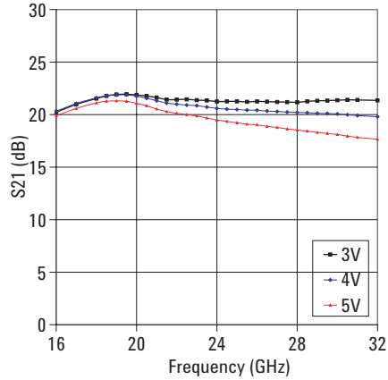
Figure 11: Gain Over Vdd
