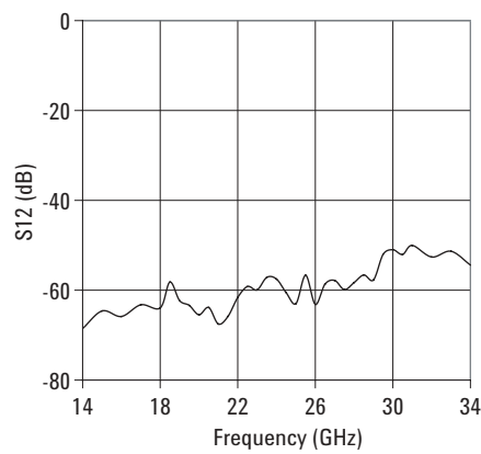
Figure 2. Typical Isolation
