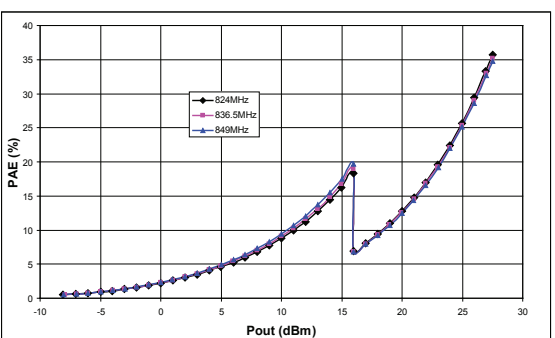
Figure 12: Efficiency vs Output Power
