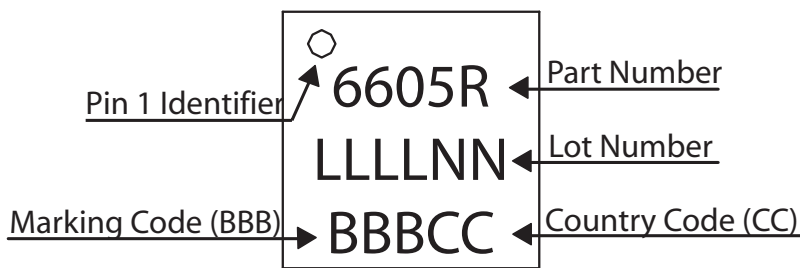
Figure 18: Branding Specification - M45 Package
