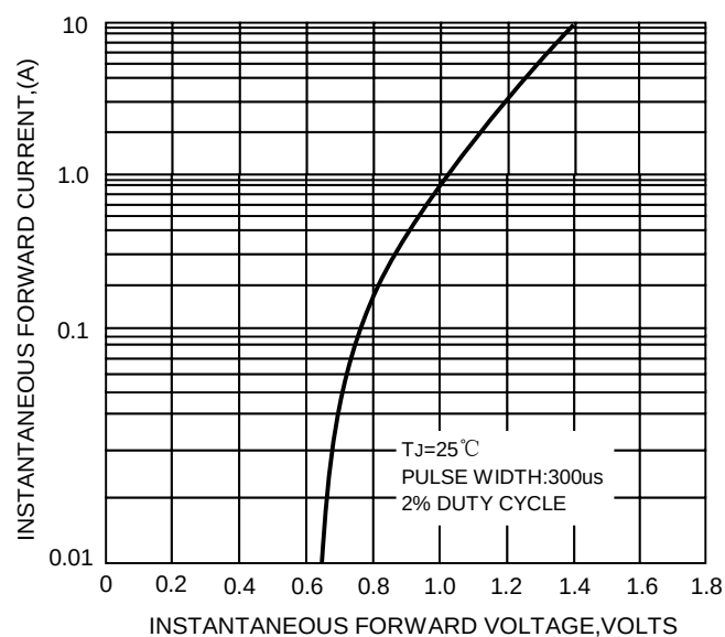
FIG.4-TYPICAL FORWARD CHARACTERISTICS
