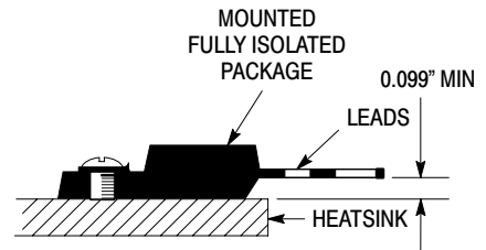
Figure 12. Screw Mounting Position for Isolation Test Number 3
