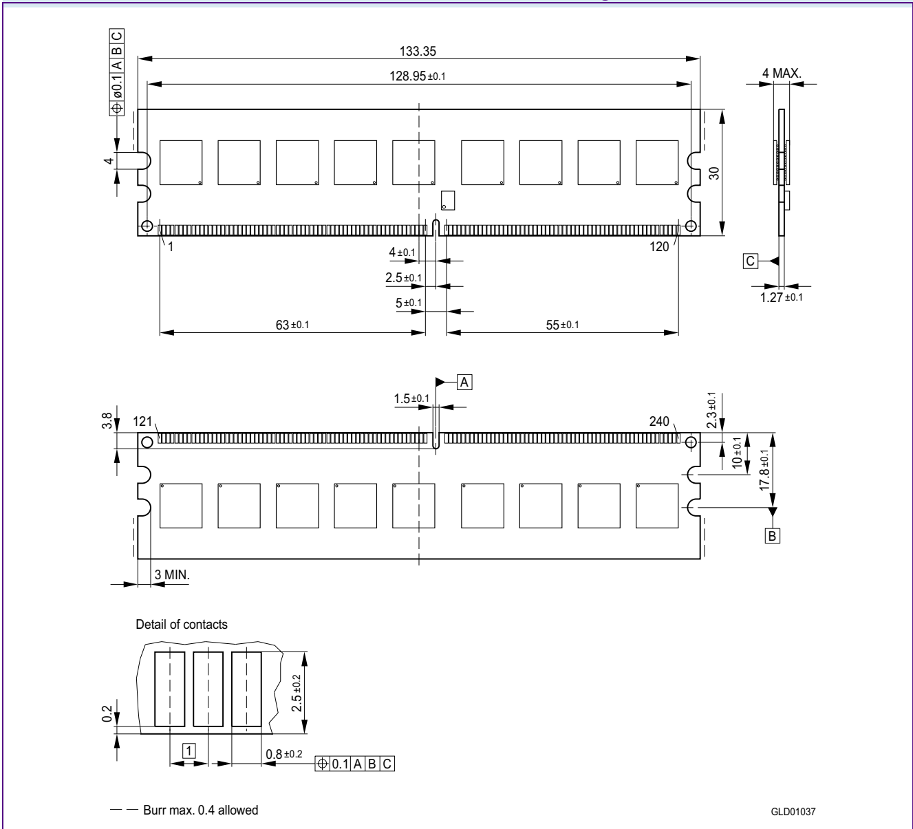
FIGURE 7 Package Outline Raw Card G L-DIM-240-7
