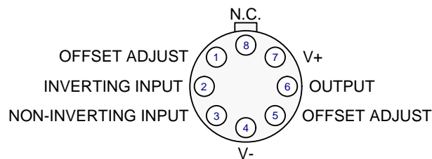
T PACKAGE
