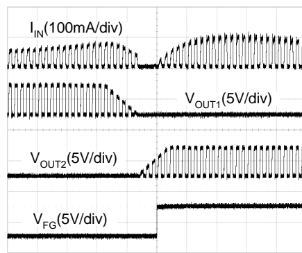
Rotation Waveform 4
