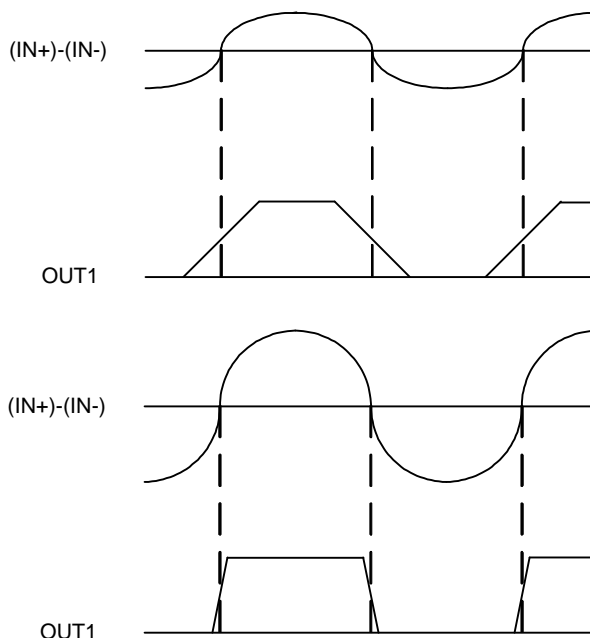
Figure 3. Differences of Output Signal Depending on the Shape of Hall Input Signal
