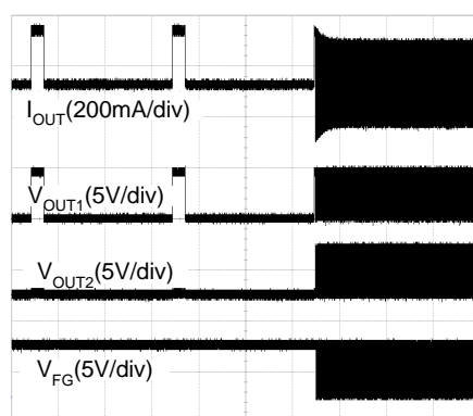
Lock Protection Waveform 2
