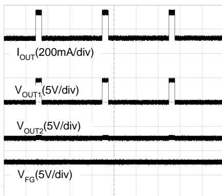
Lock Protection Waveform 1
