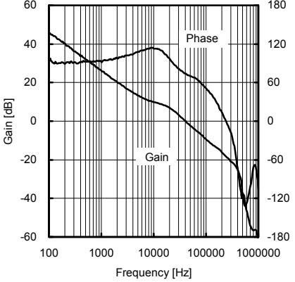
Fig.39 Frequency response 5 (VCC=7.4V, Io=300mA)
