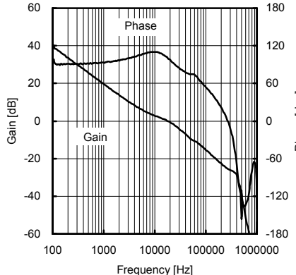
Fig.36 Frequency response 2 (VCC=5.0V, Io=300mA)
