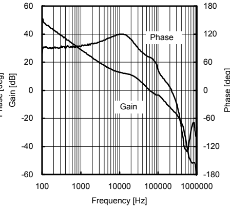
Fig.43 Frequency response 9 (VCC=10V, Io=900mA)
