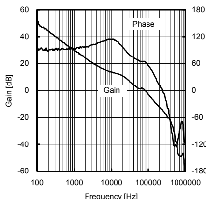
Fig.42 Frequency response 8 (VCC=10V, Io=300mA)
