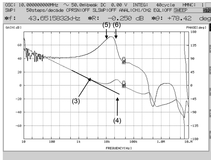
Fig.52 Example of DC/DC converter frequency property (Measured with FRA5097 by NF Corporation)
