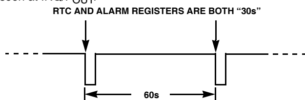
FIGURE 14. \overline{\text{IRQ}}/\text{F}_{\text{OUT}} WAVEFORM
