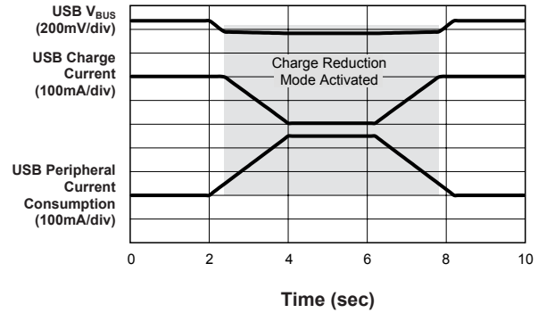
USB Charge Current vs. Time ( R_{USBSET} = 8.06k\Omega )
