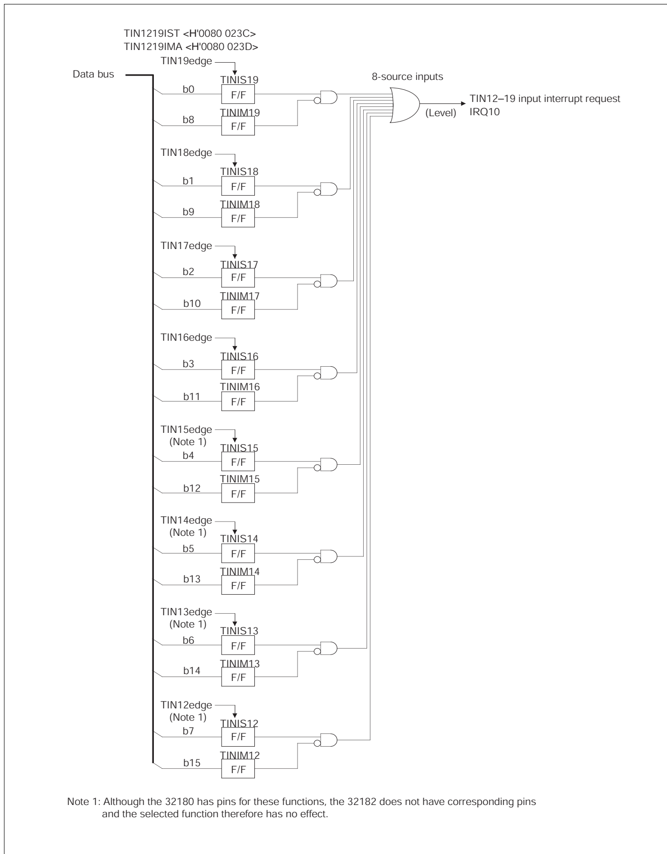
Figure 10.2.14 Block Diagram of TIN12-19 Input Interrupt Request
