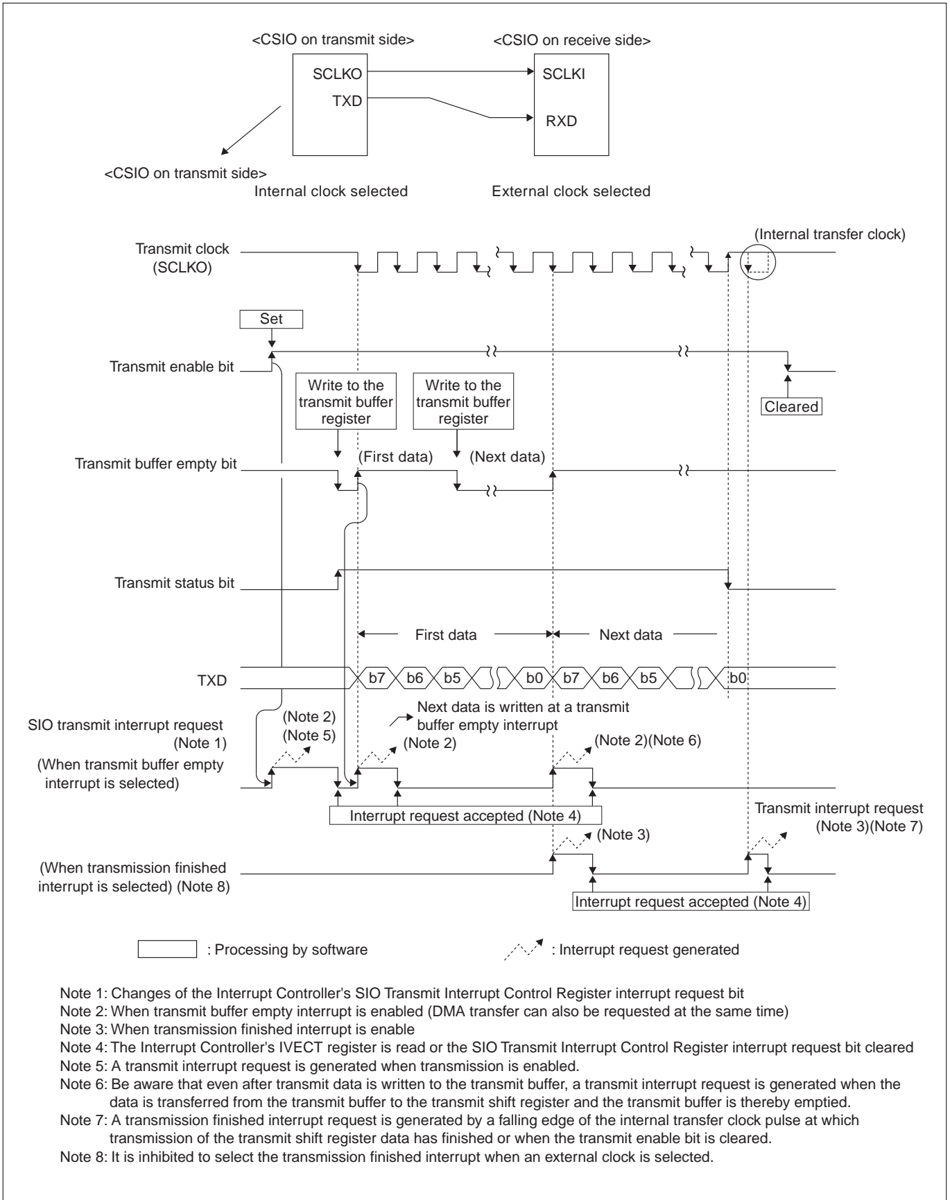
Figure 12.3.4 Example of CSIO Transmission (Transmitted Successfully)
