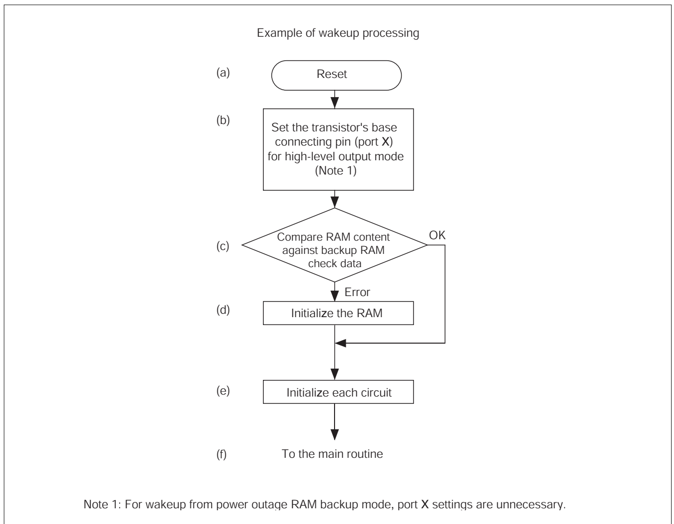
Figure 17.4.1 Wakeup Processing
