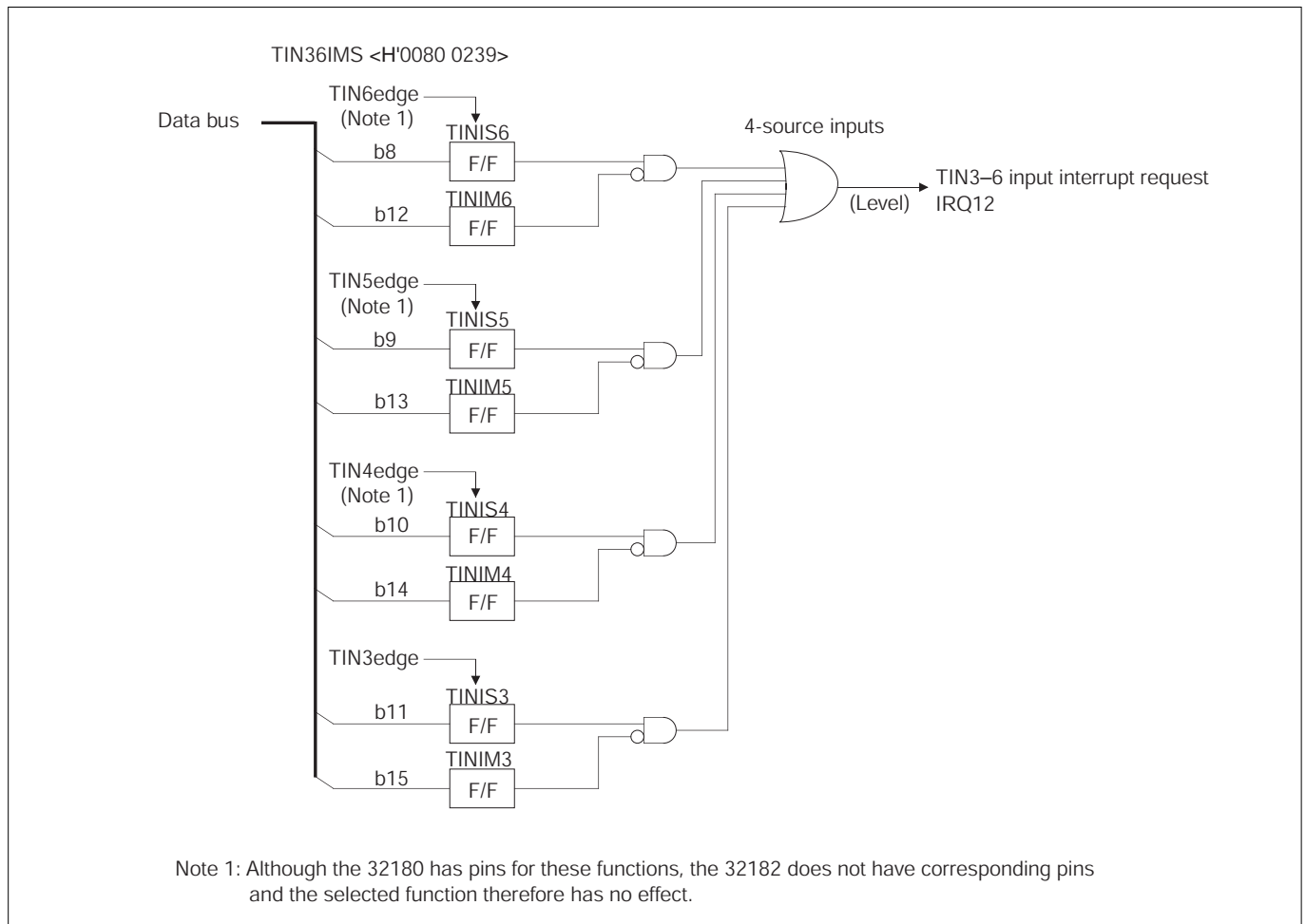
Figure 10.2.13 Block Diagram of TIN3–6 Input Interrupt Request
