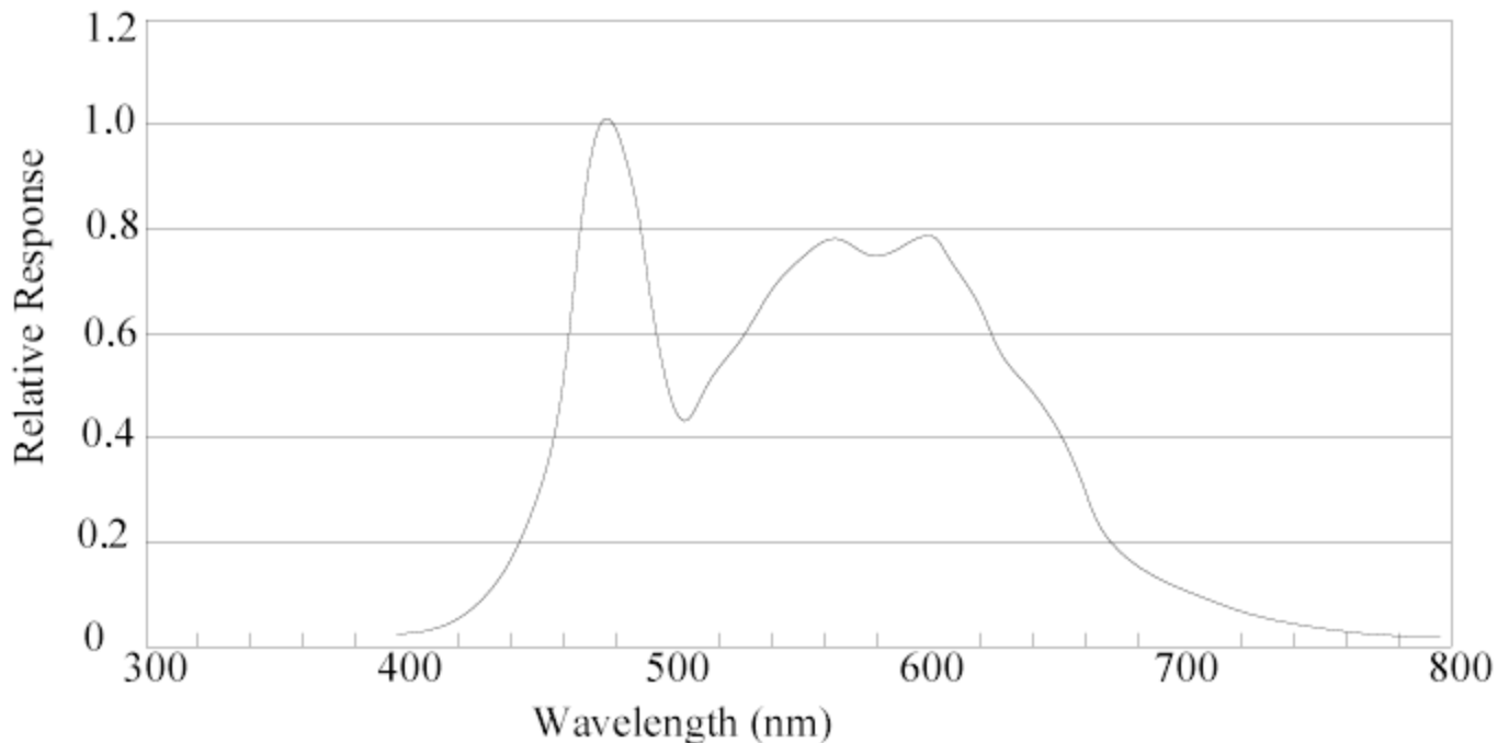
Fig.1 WHITE LED Spectrum VS. WAVELENGTH
