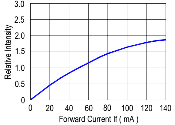
FIG. 2 Relative Total Flux vs. Forward Current ( Ta = 25 °C )
