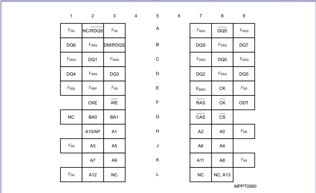
FIGURE 1 Chip Configuration for ×8 components, PG-TFBGA-60 (top view)
