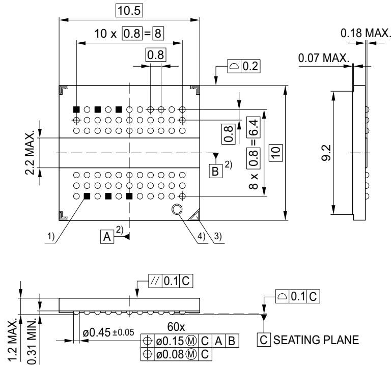
FIGURE 9 Package Outline PG-TFBGA-60
