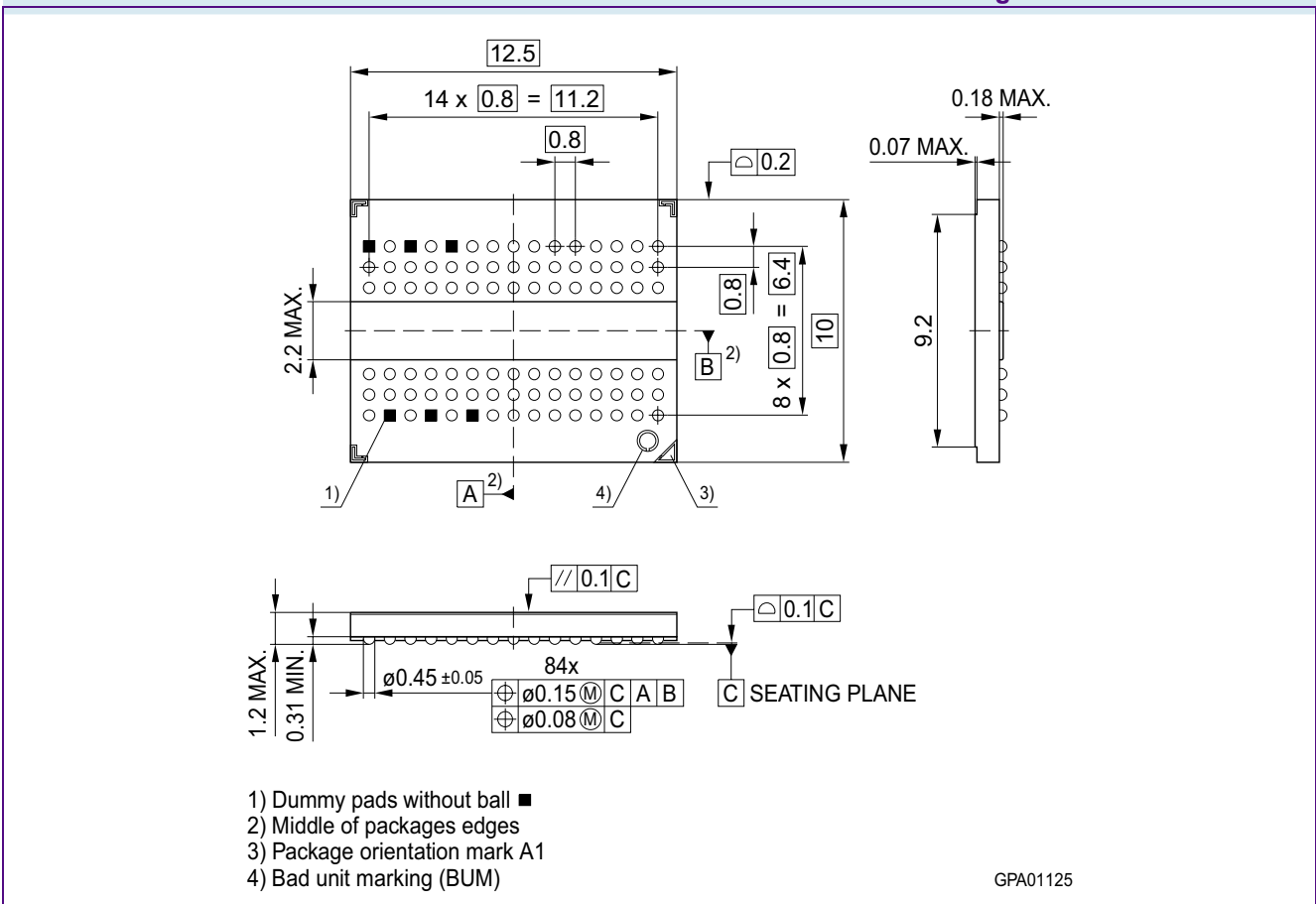
FIGURE 8 Package Outline PG-TFBGA-84
