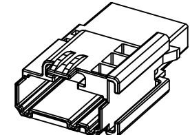
OPTION "B" VIEWED FROM MATE SIDE
