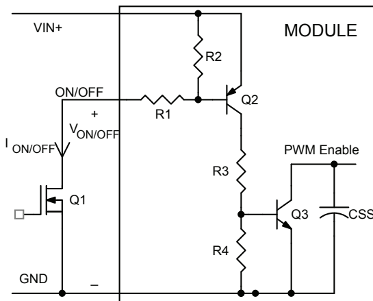
Figure 27. Circuit configuration for using positive logic On/Off.
