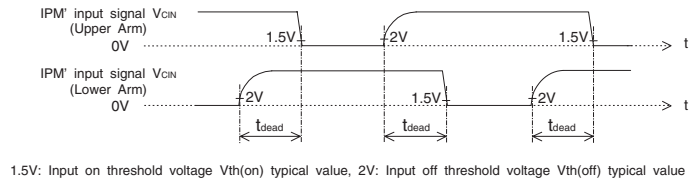
1.5V: Input on threshold voltage V_{th(on)} typical value, 2V: Input off threshold voltage V_{th(off)} typical value
