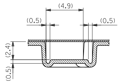
SECT. W-W
