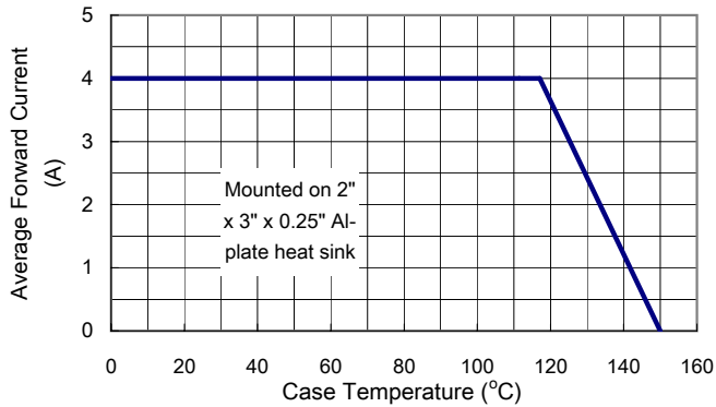
FIG 1 Maximum Derating Curve for Output Current
