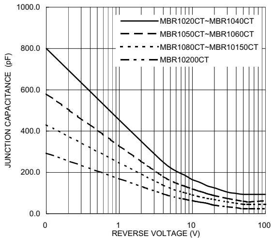
FIG. 5-TYPICAL JUNCTION CAPACITANCE
