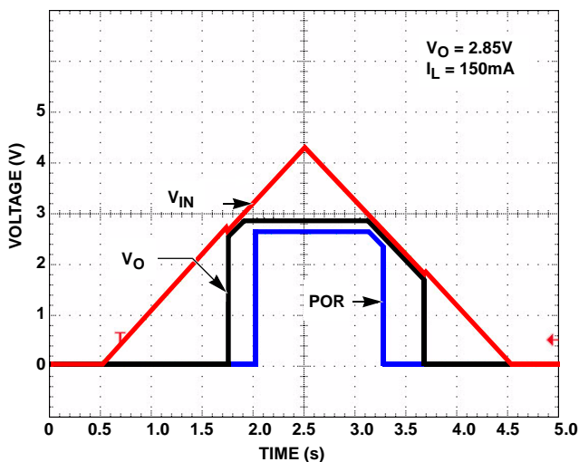
FIGURE 12. POWER-UP/POWER-DOWN
