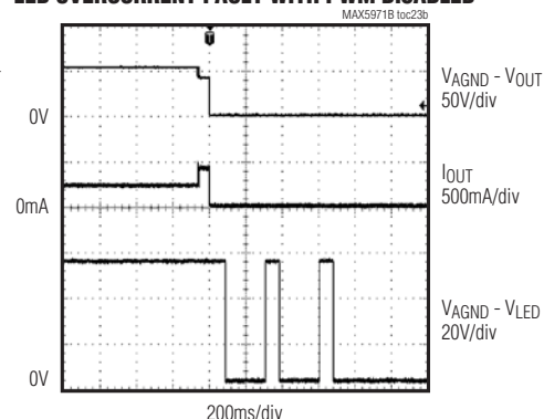
LED OVERCURRENT FAULT WITH PWM DISABLED
