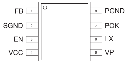
MSOP-8
