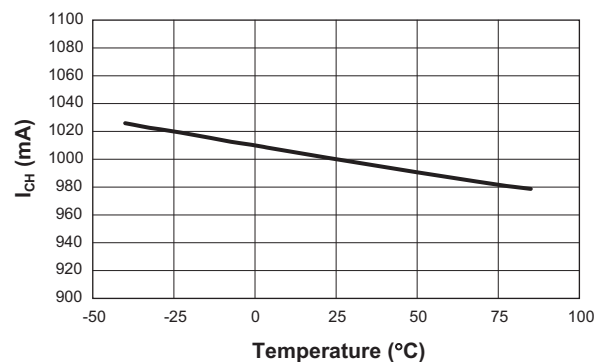
Constant Charging Current vs. Temperature (ADPSET = 8.06k \Omega )
