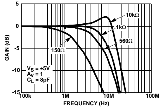
FIGURE 12. FREQUENCY RESPONSE FOR VARIOUS R_L
