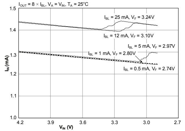
I_{IN} Supply Current (8 LEDs)
