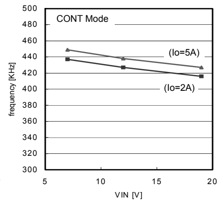
Fig. 18 VIN-frequency (Vo1=5.0V)
