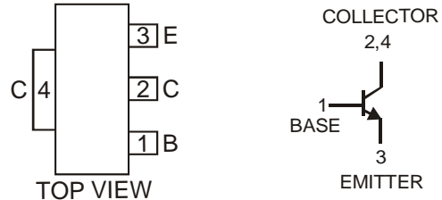
Schematic and Pin Configuration
