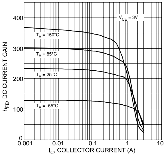
Fig. 3 Typical DC Current Gain vs. Collector Current (2DD1664R)
