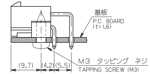
基板取付推奨寸法 RECOMMENDED INSTALLATION PATTERN
