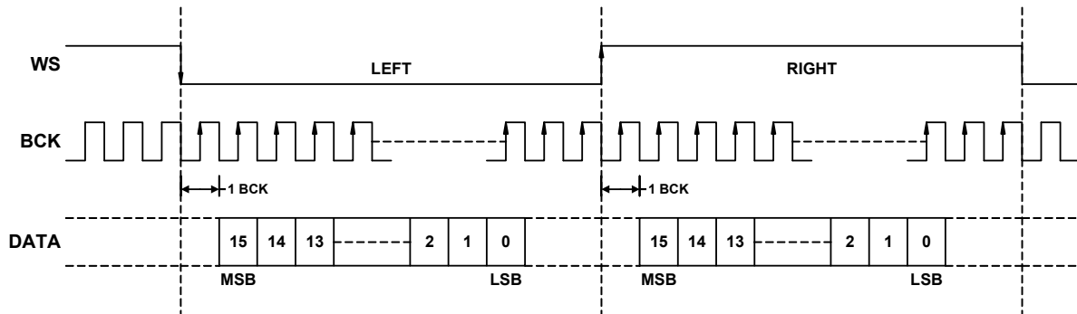
Fig.3 I2S format
