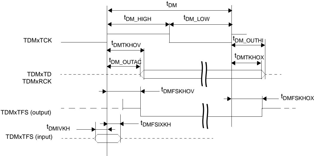
Figure 21. TDM Transmit Signals
