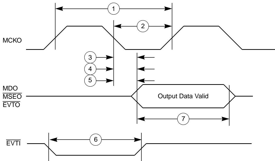
Figure 25. Nexus Timings
