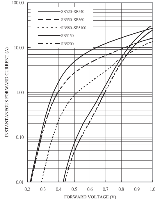
FIG. 2-TYPICAL FORWARD CHARACTERISTICS
