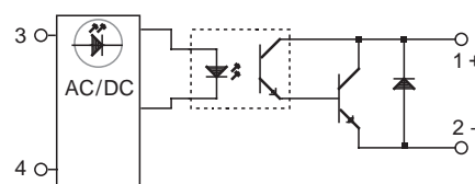
Figure 3 — DX relays
