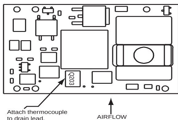
Figure 43. HW 6.6A-12A-Series Temperature Measurement Location (Top View).
