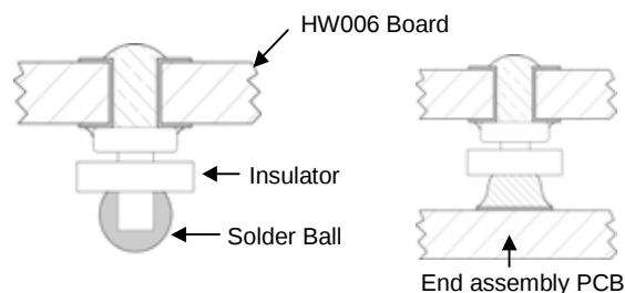
Figure 50. Column Pin Connector Before and After Reflow Soldering.
