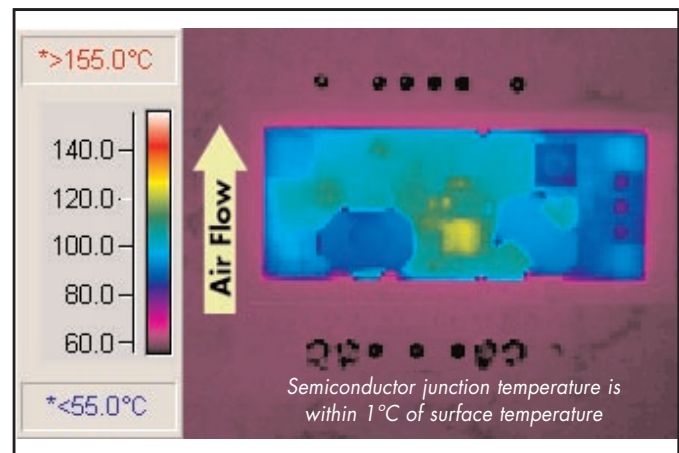
Figure 6: Thermal plot of converter at 10 amp load current with 55°C air flowing at the rate of 200 LFM. Air is flowing across the converter sideways from pin 3 to pin 1 (nominal input voltage).
