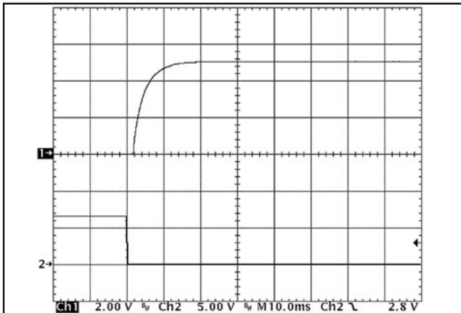
Figure 9: Turn-on transient at full load (resistive load) (10 ms/div). Ch 1: V_{out} (2V/div) Ch 2: ON/OFF input (5V/div)
