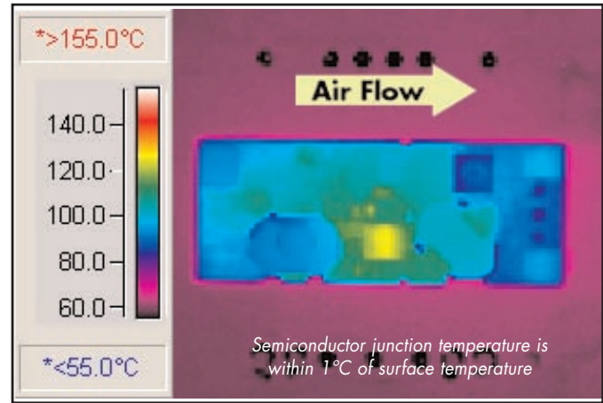
Figure 8: Thermal plot of converter at 10 amp load current with 55°C air flowing at the rate of 200 LFM. Air is flowing across the converter from input to output (nominal input voltage).
