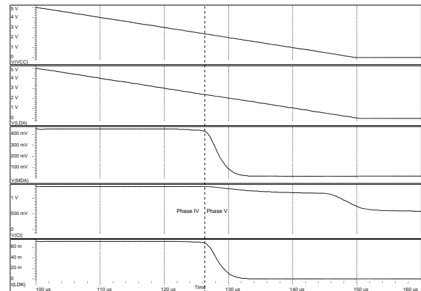
Figure 2: Turn-off behaviour
