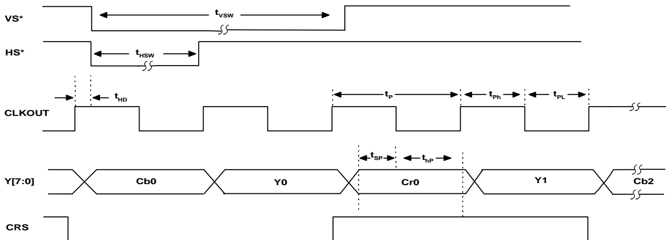
Figure 12: Timing Diagram (M[2:0] = 1, OF = 1, H Start = 0)
