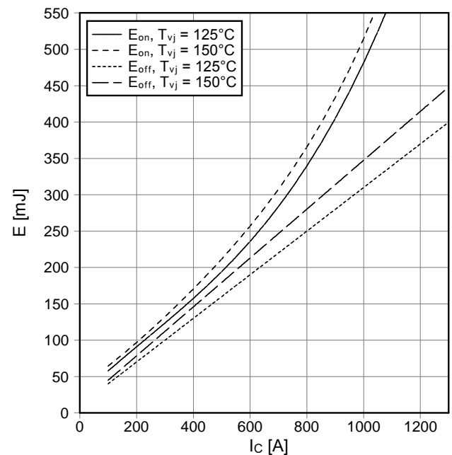
Schaltverluste IGBT-Wechselr. (typisch) switching losses IGBT-inverter (typical) E_{on} = f(I_C), E_{off} = f(I_C) V_{GE} = \pm 15\text{ V}, R_{Gon} = 1\ \Omega, R_{Goff} = 2.7\ \Omega, V_{CE} = 900\text{ V}
