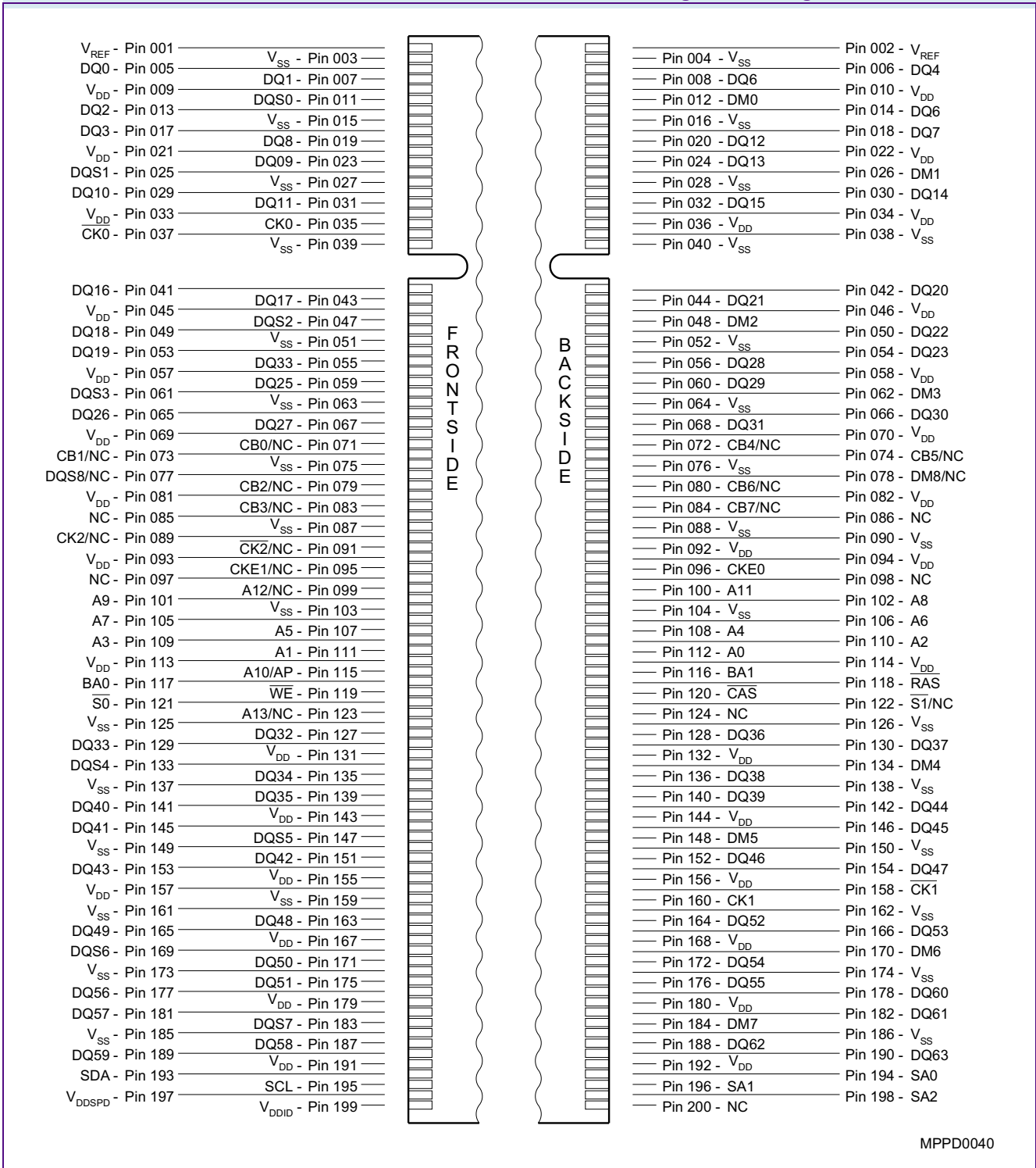
FIGURE 1 Pin Configuration Diagram 200-Pin SO-DIMM
