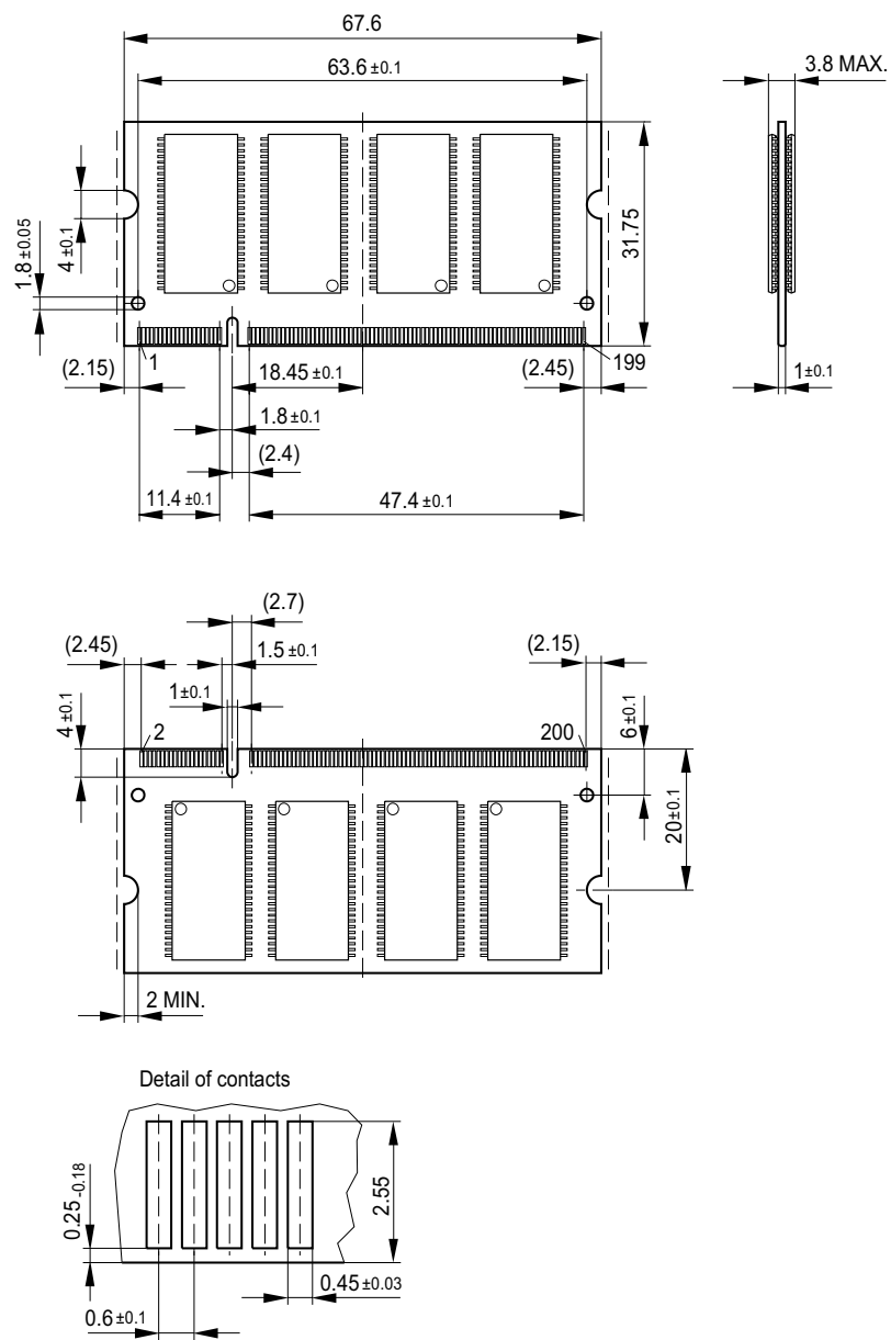
Package Outline SO-DIMM Raw Card A (L-DIM-200-6)
