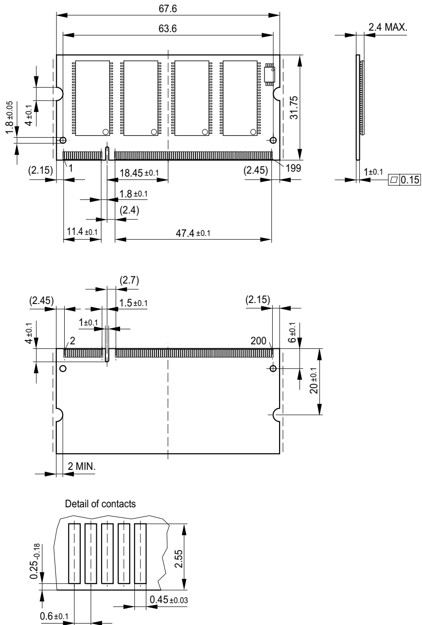
FIGURE 5 Package Outline SO-DIMM Raw Card C (L-DIM-200-11)
