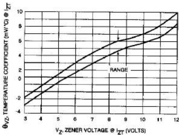
Fig. 5-UNITS TO 12 VOLTS
