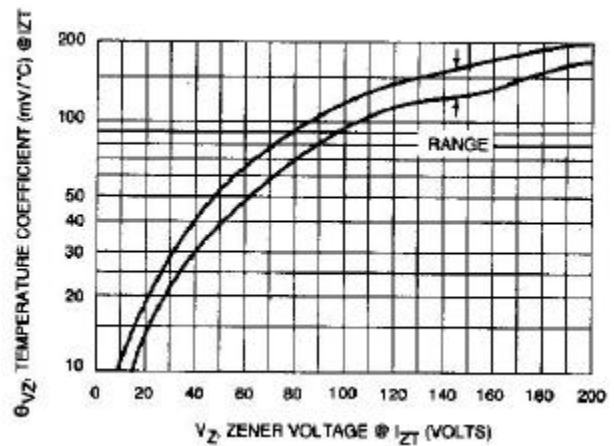
Fig. 6-UNITS 10 TO 200 VOLTS
