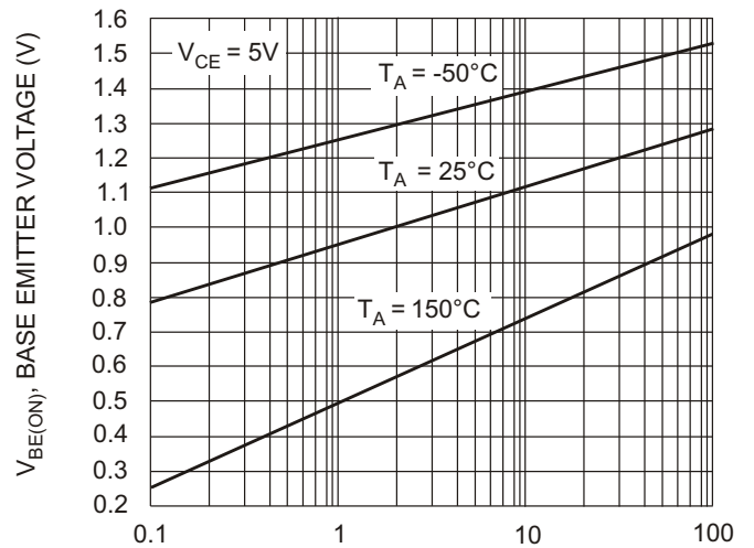
Fig. 4, Base Emitter Voltage vs. Collector Current
