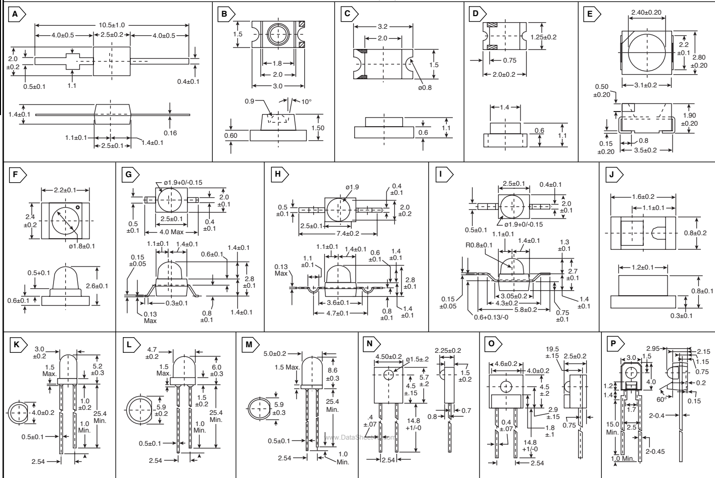
DIMENSIONS (mm)
