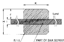
LAND PATTERN
