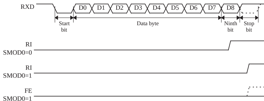
Figure 5 Enhanced UART timing diagram in mode 2 and 3
