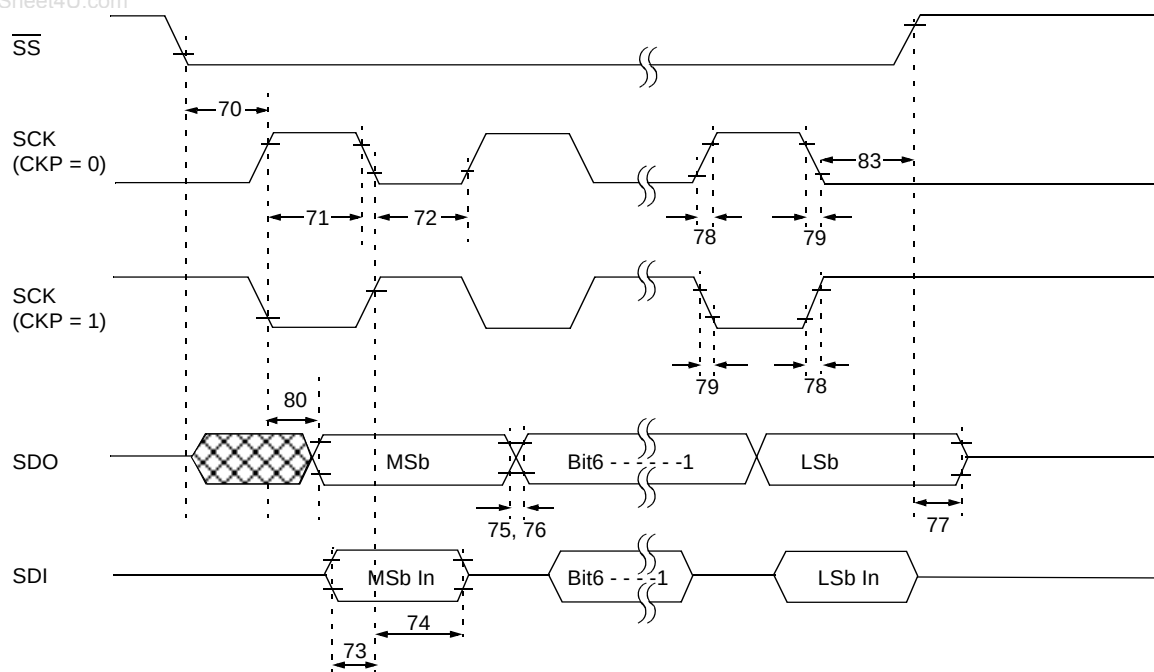
FIGURE 15-13: SPI SLAVE MODE TIMING (CKE = 0)
