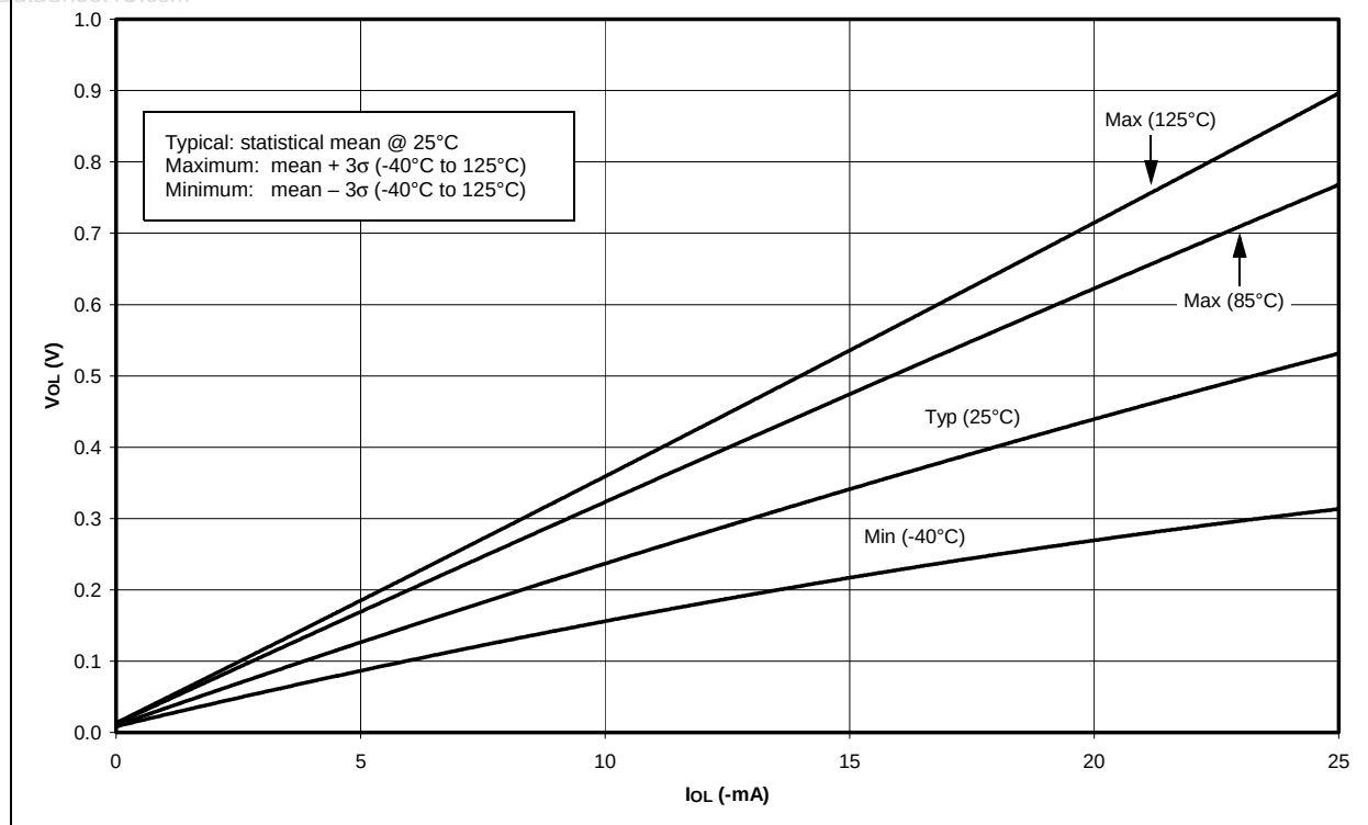
FIGURE 16-17: TYPICAL, MINIMUM AND MAXIMUM V_{OL} vs. I_{OL} ( V_{DD} = 5V , -40^{\circ}C TO 125^{\circ}C )
