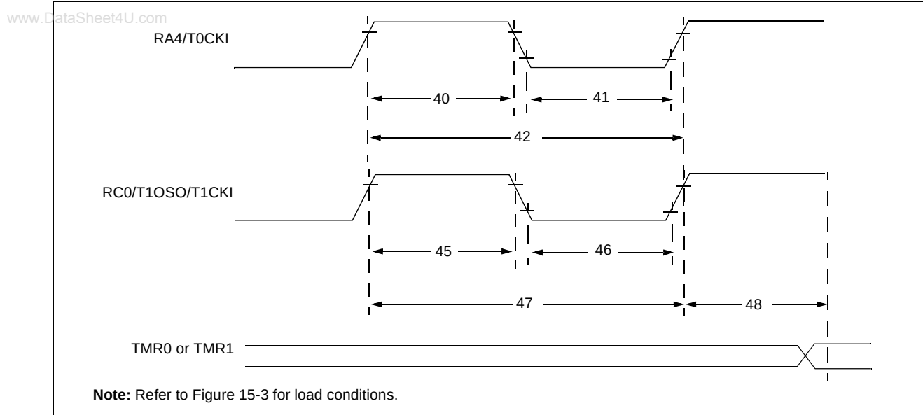
FIGURE 15-8: TIMER0 AND TIMER1 EXTERNAL CLOCK TIMINGS
