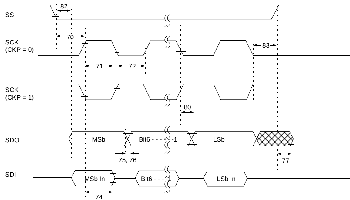
FIGURE 15-14: SPI SLAVE MODE TIMING (CKE = 1)
