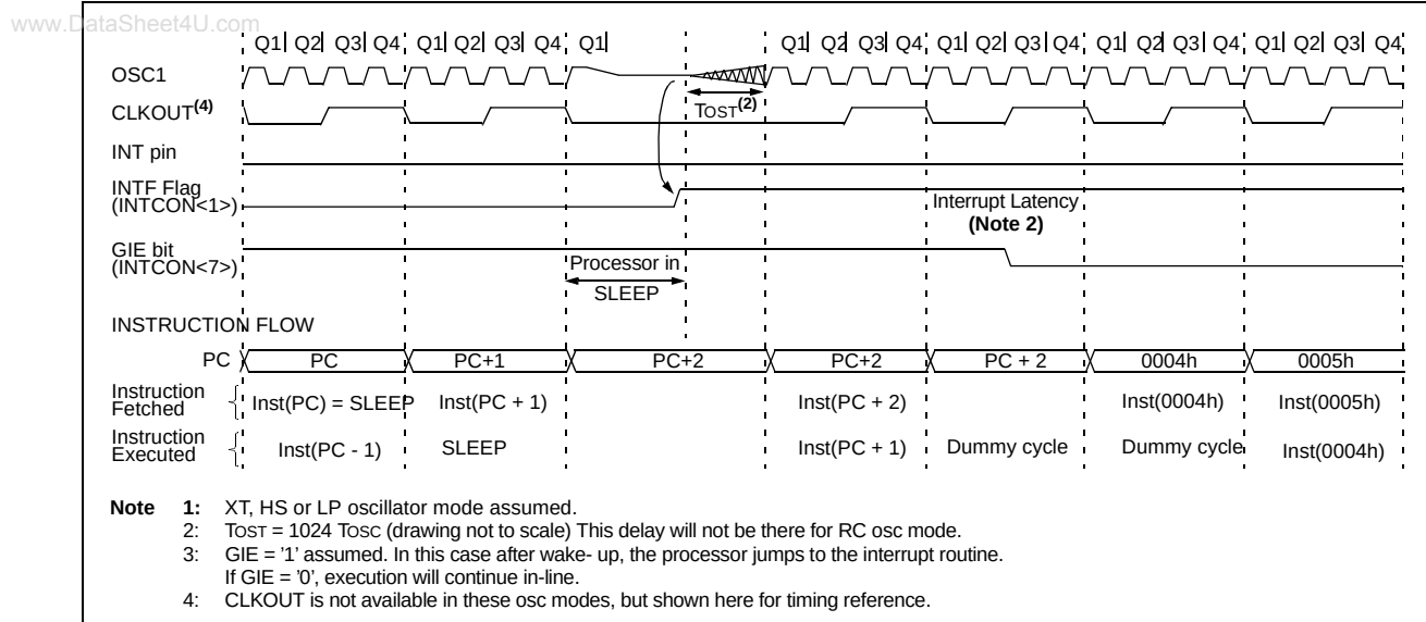
FIGURE 12-12: WAKE-UP FROM SLEEP THROUGH INTERRUPT
