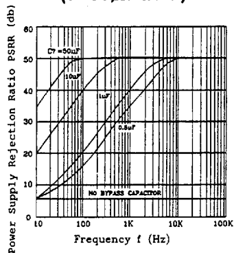
Power Supply Rejection Ratio vs. Frequency (V + =6V, A v =26dB)
